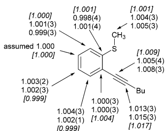
Figure 2. Experimental and B3LYP-D3/6-31+G**/PCM(toluene)-predicted (italicized and in brackets) 13 C KIEs ( k 12 / k 13 ) at 85 °C for the thioboration reaction of 1a with ClBcat. The 95% confidence limits on the last digit are shown in parentheses with the experimental values.
