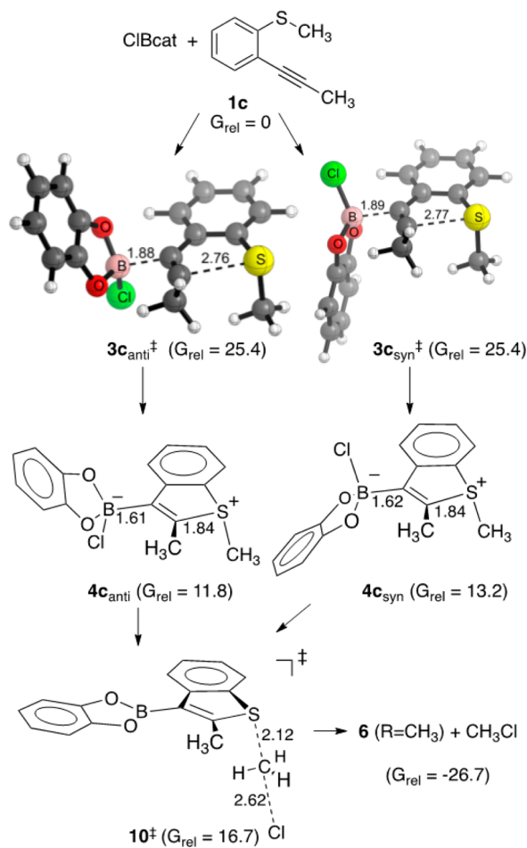
Scheme 2. Calculated Mechanism (B3LYP-D3/6-31+G**/PCM(Toluene)) for the Reaction of 1c with ClBcat
