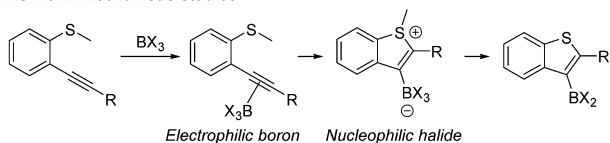
Figure 1. Previous work on catalyst-free borylative cyclizations and this work on mechanistic elucidation of the thioboration reaction.
