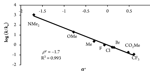
Figure 3. Hammett study showing correlation between log( k / k 0 ) and σ + at 100 °C.
