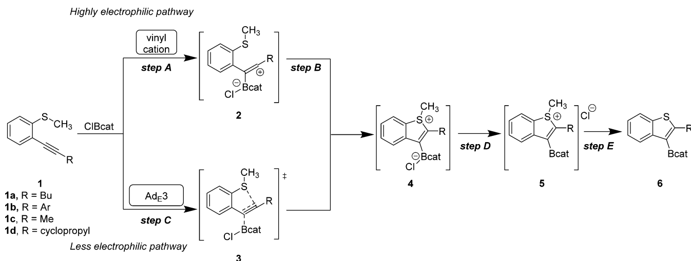
Scheme 1. Two Possible Mechanistic Pathways for Thioboration with ClBcat
