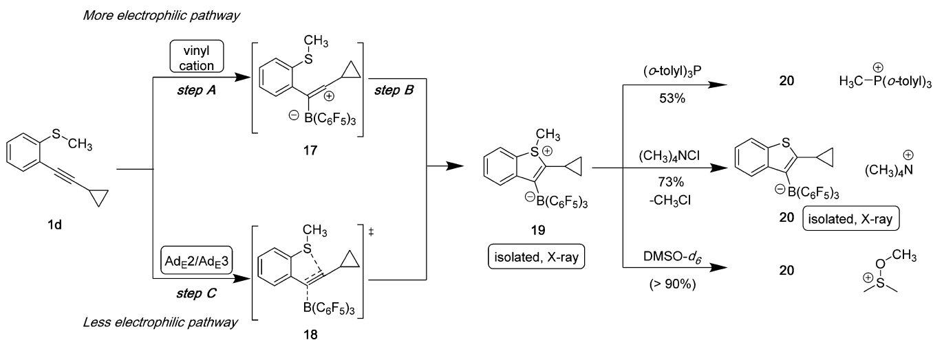
Scheme 3. Two Possible Mechanisms for Thioboration with \text{B}(\text{C}_6\text{F}_5)_3 and Isolation of Intermediates
